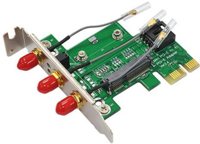
Half Size mPCIe to PCIe Adapter
