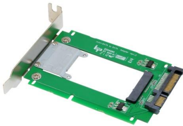
mini-SATA to SATA Adapter SSDMC module
