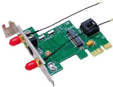
M.2 Wireless Card to PCIe Adapter M2P2H
