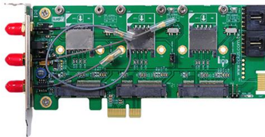
Triple mPCIe to PCIe Adapter
